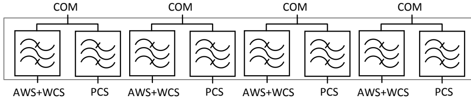
Block diagram. Quad unit.
